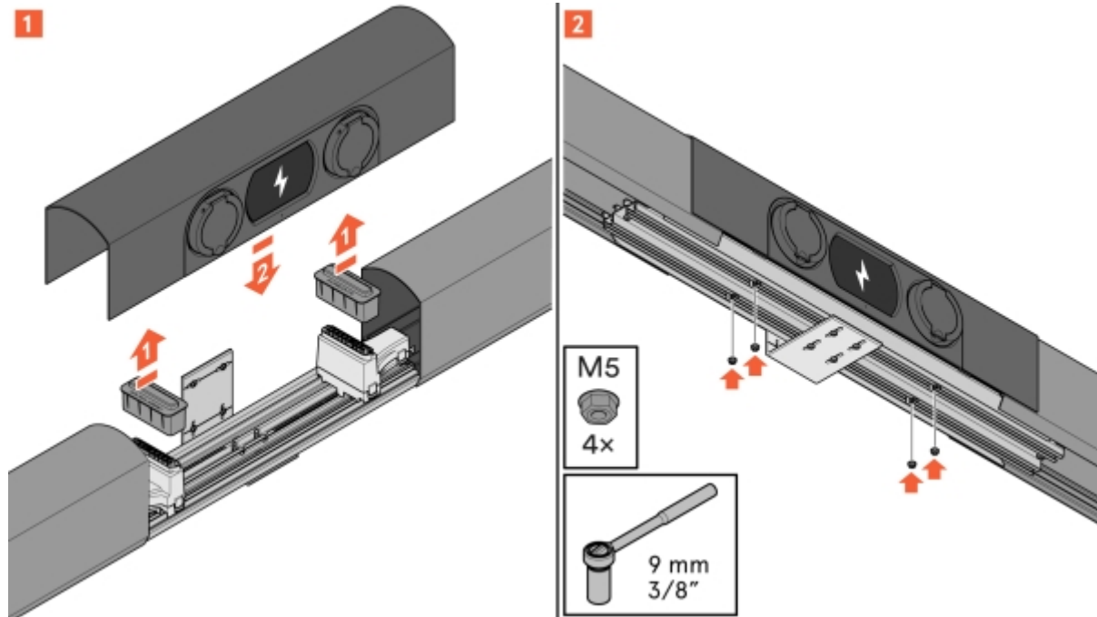
Illustration 41: Montage du ChargePod
