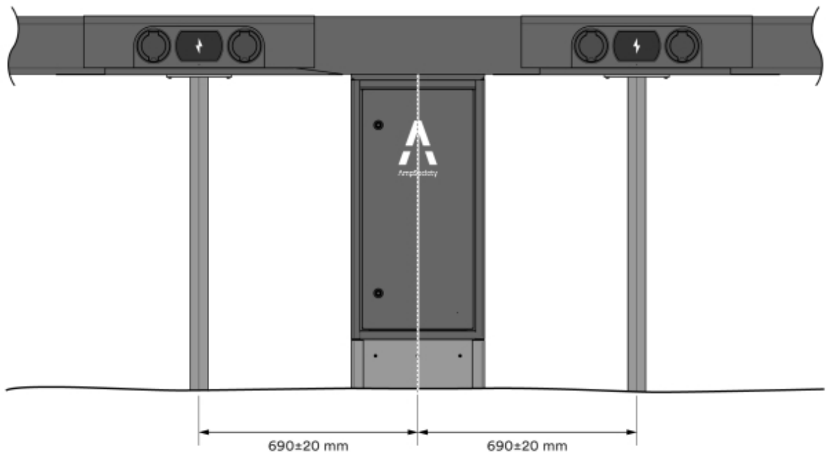
Illustration 8: Cotes - deux directions
