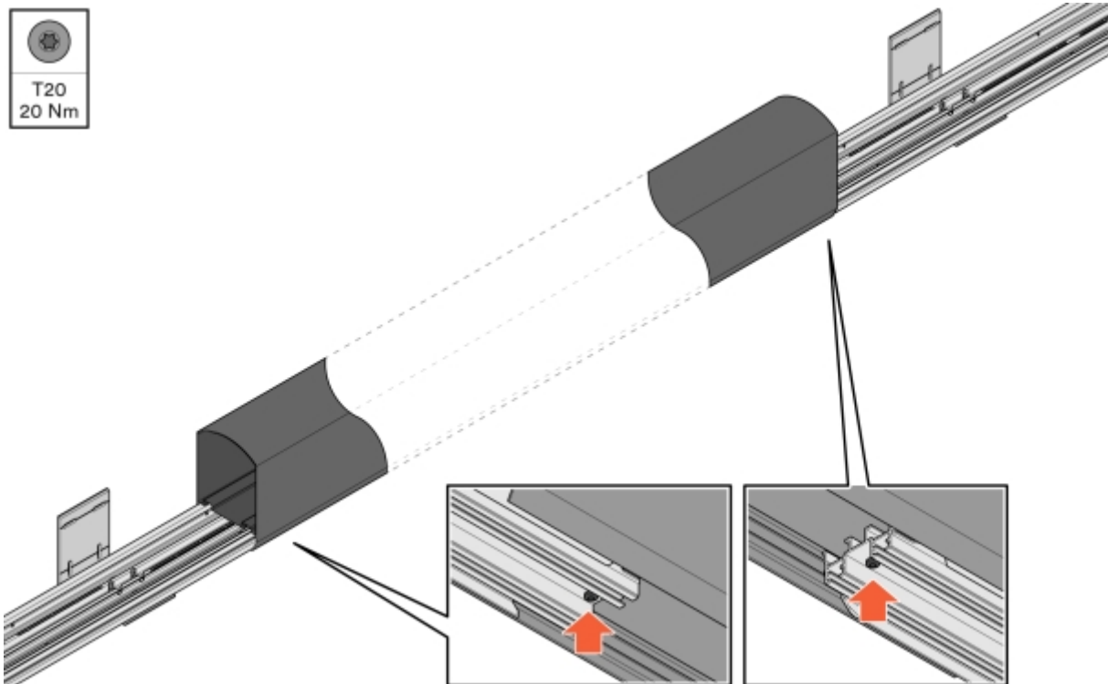
Illustration 36: Fixation de la ConnectBar
