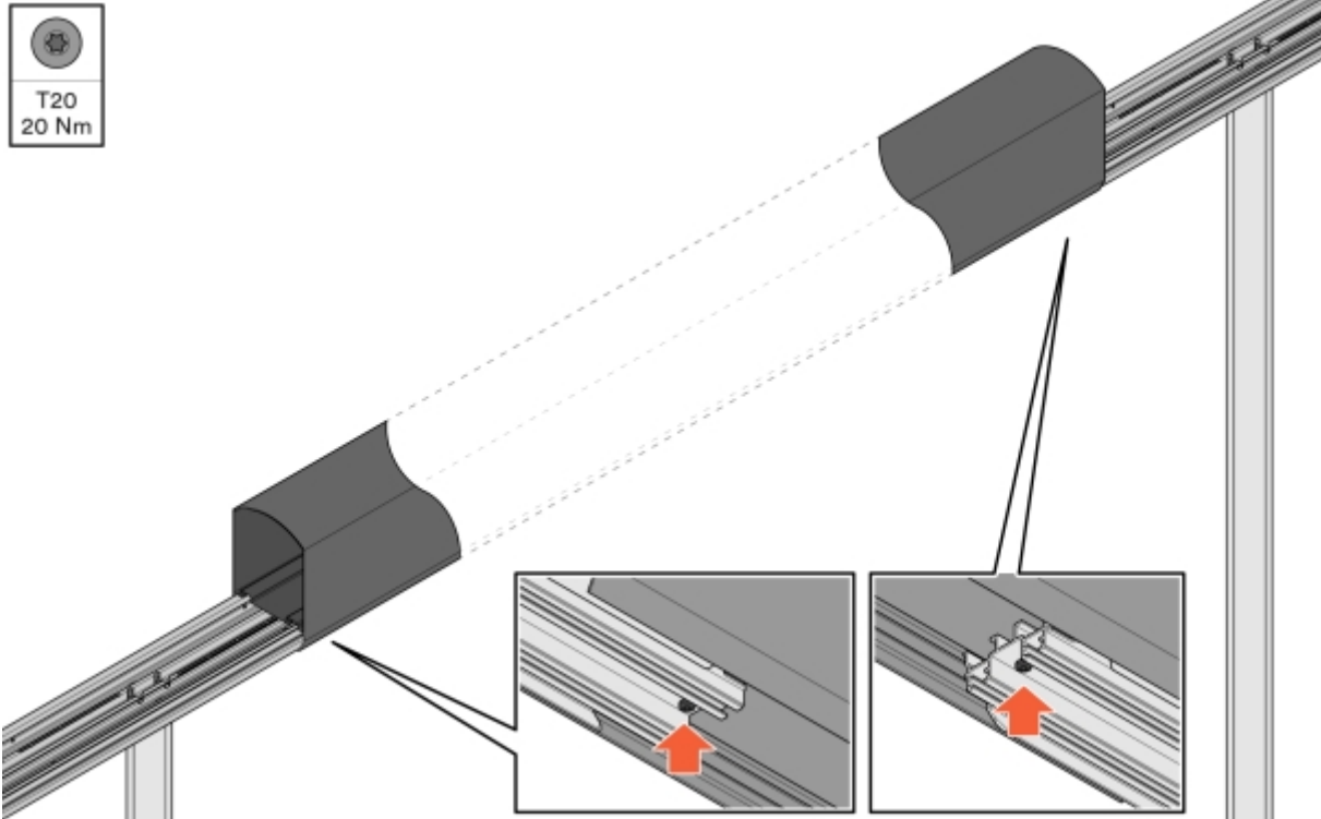
Illustration 23: Fixation de la ConnectBar
