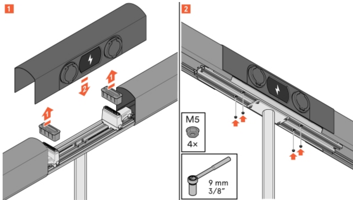
Illustration 28: Montage du ChargePod
